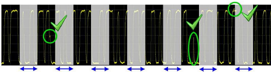
Figure 10. InfiniiVision 30000T X-Series with 1,000,000 waveforms/second. A short dead time increases the probability of capturing infrequent events.
